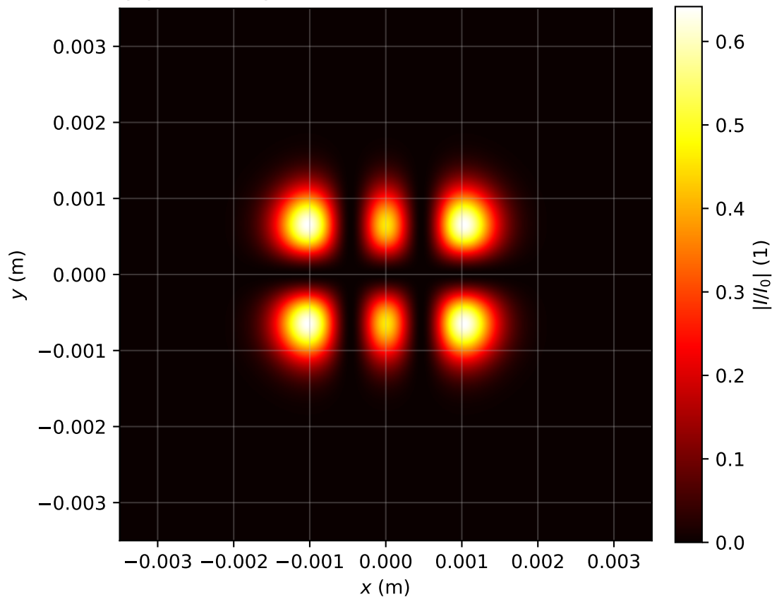
Intensity profile I(x, y, z = 1.672)/I_0 , P_{in}=0.5P_{cr} , artificial time
